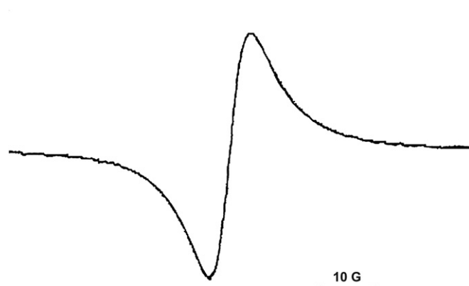
Figure 2. EPR spectra of the CH 2 Cl 2 solution containing the Pd(0)/Naph 2.2+ material recorded at 293 K.
