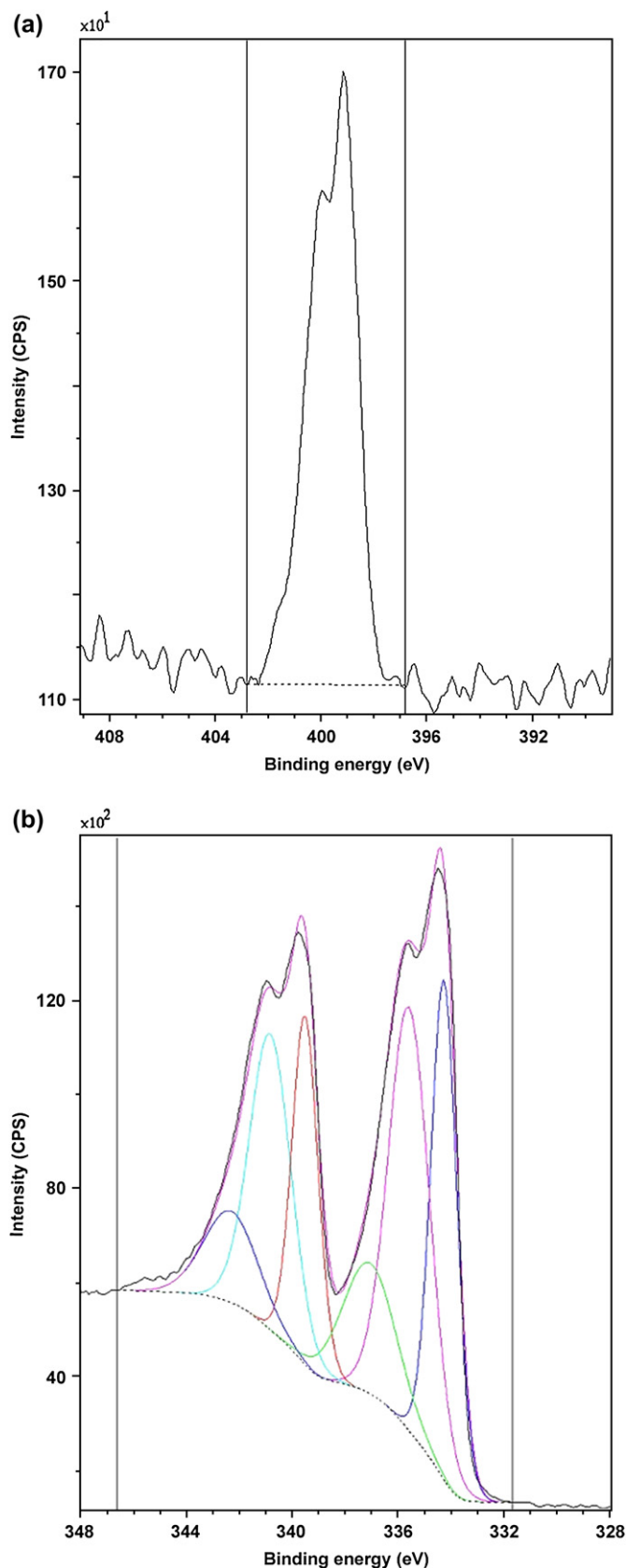
Figure 6. XPS analysis of the Pd/Napht 2.2+ nanomaterial: the binding energy spectrum of (a) N 1s and (b) Pd 3d.
